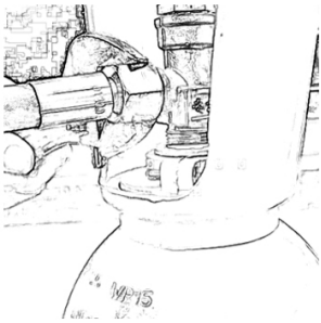
Tighten the gas pipe and cylinder with a wrench
